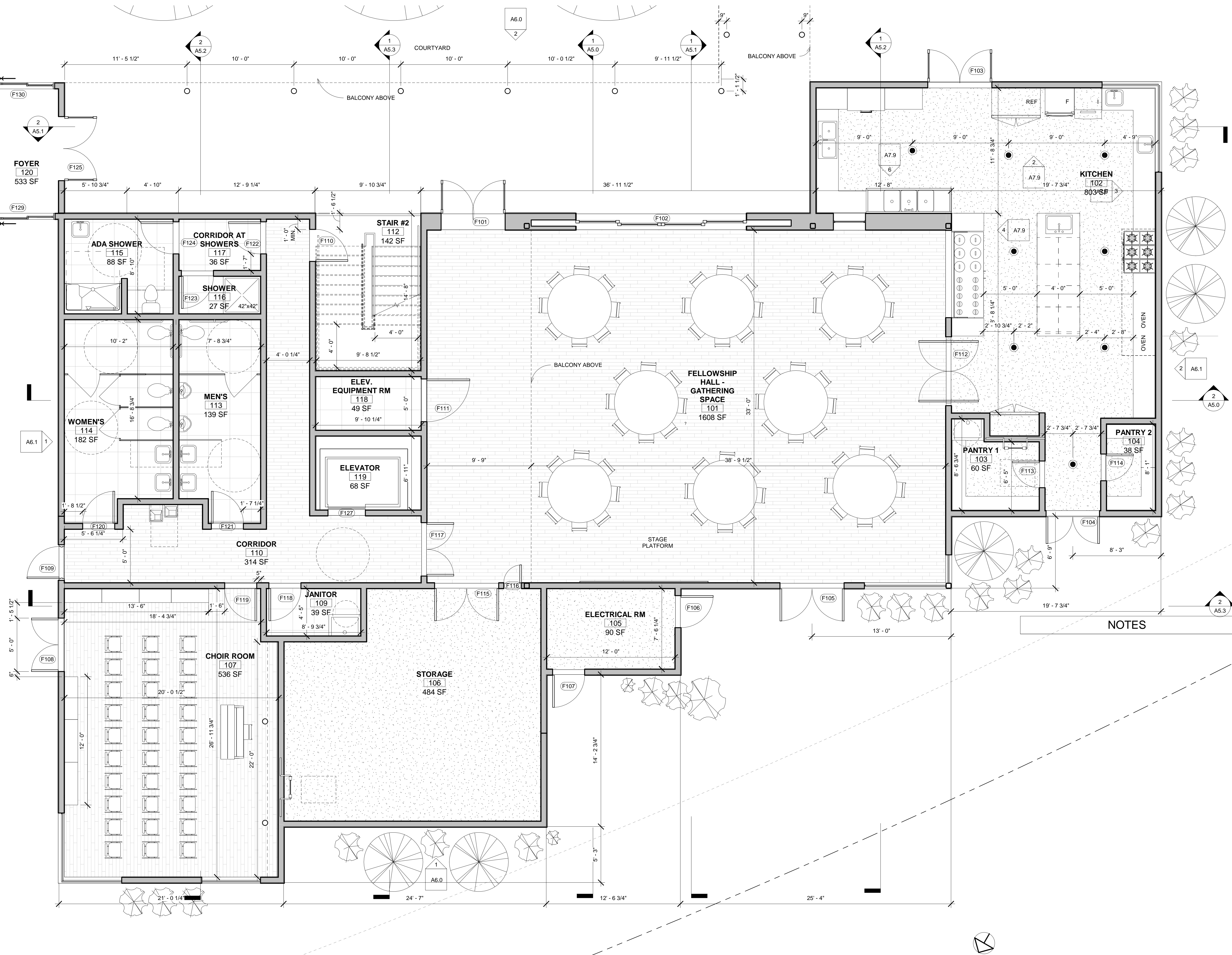
1 (N) FELLOWSHIP HALL FIRST FLOOR 1/4" = 1'-0"
