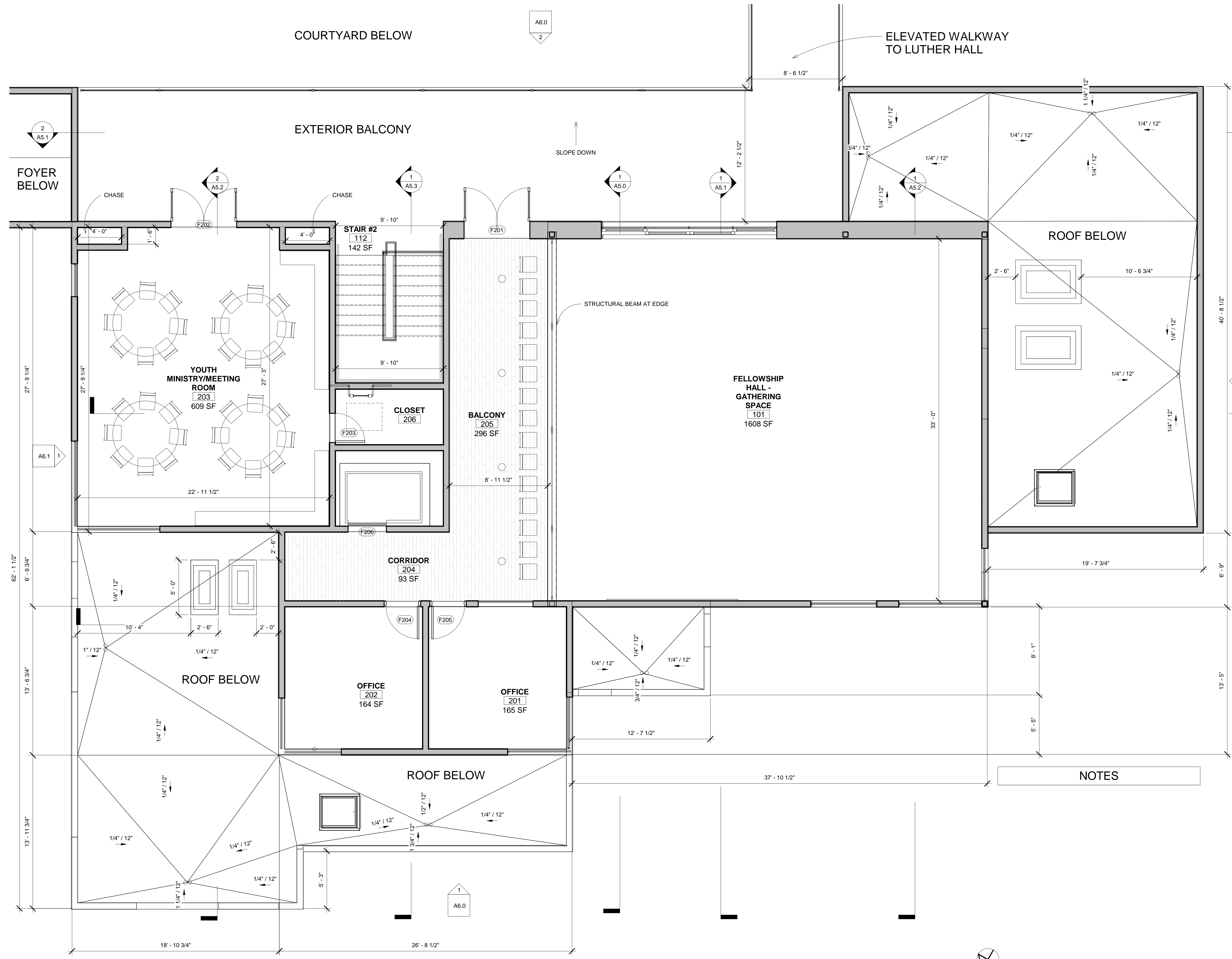
1 (N) FELLOWSHIP HALL SECOND FLOOR 1/4" = 1'-0"
